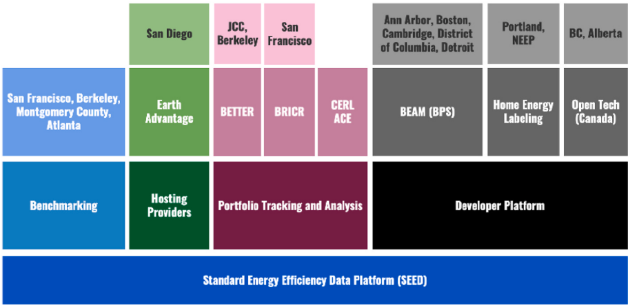
Fig. 10. SEED has been leveraged by various additional use cases to further standardize building data management for benchmarking and BPS.
